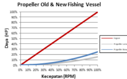
Figure 12: Graph of the Difference between old and new propeller matching points
