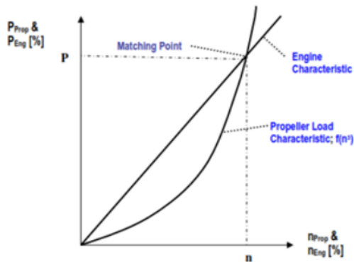
Figure 5: Matching point engine and propeller
