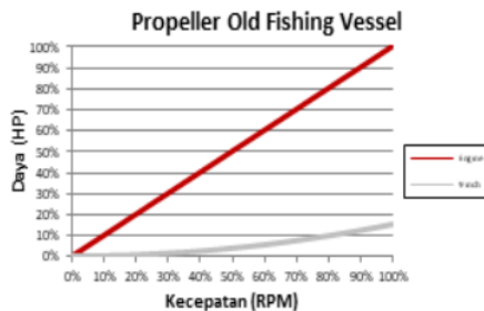
Figure 11: Graph of old fishing vessel propeller matching
