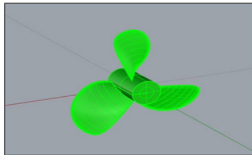
Figure 8: Model B-Series propeller type B3-50 on old fishing vessel
