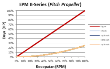
Figure 10: Graph of matching propeller B-Series with pitch propeller 14.00 inch; 14.25 inch; 14.5 inch; and 14.75 inch
