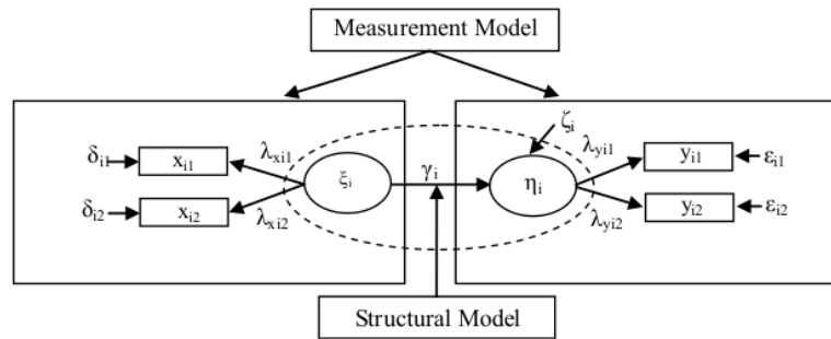
Fig.1 A first-order structural equation model demarcated into measurement model.
