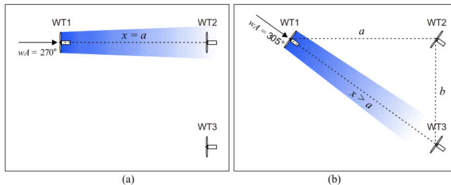
Fig. 2. Wake Interaction Dynamics
