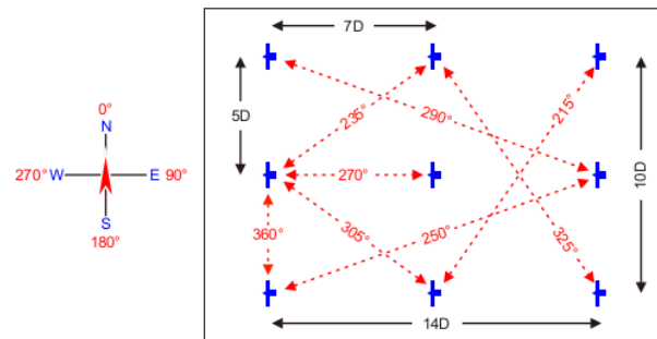
Fig. 3. Wind Farm Layout
