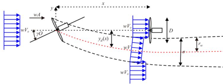
Fig. 6. Adjustment of Wake Bending by Controlling the Yaw Offset Angle
