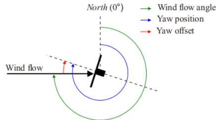
Fig. 5. Wind Turbine Yaw Angle Variables
