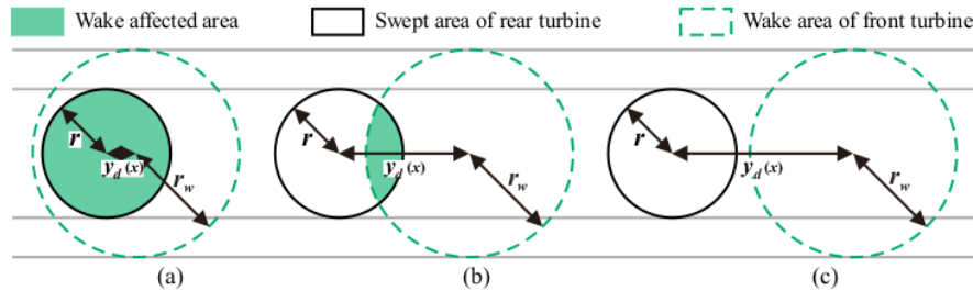
Fig. 7. Front View Wake Interaction
