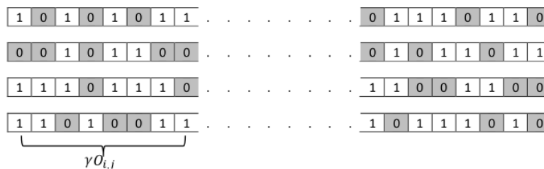
Fig. 9. Population Representation
