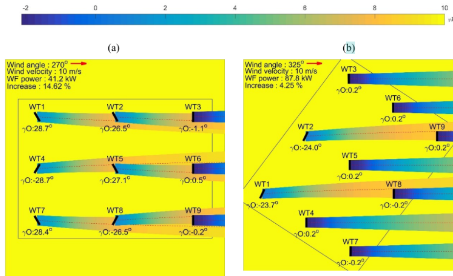
Fig. 11. Optimal Combination of Yaw offset and Wind Flow Velocity Distribution, (a) \omega A = 270^\circ , (b) \omega A = 325^\circ
