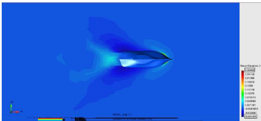
Figure 5 The wave pattern of hullvane ship model with angle of attack 2^\circ at Fn 0.527
