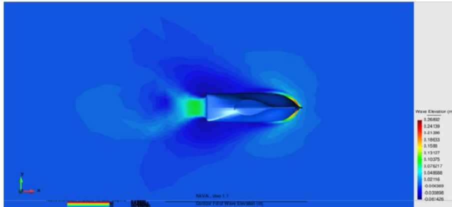
Figure 4 The wave pattern of original ship model in Fn 0.527
