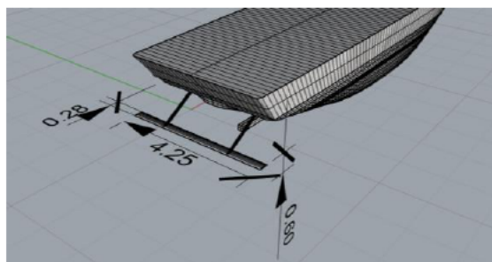
Figure 2 30 GT Fish Boat Model with hull vane
