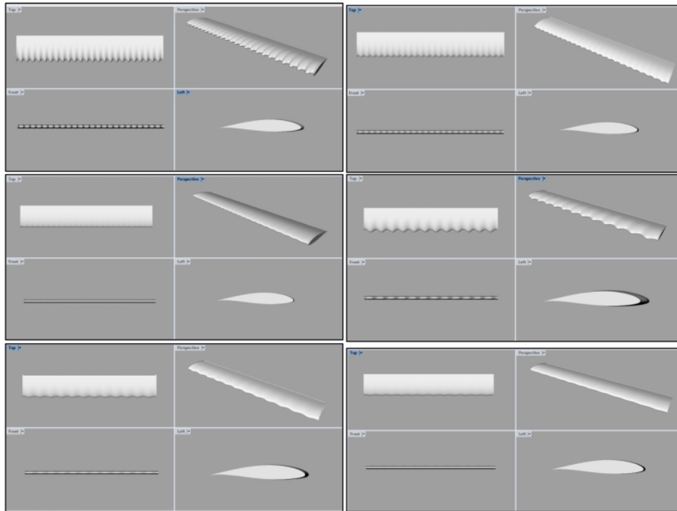
Figure 2. Model variation of leading edge protuberances
