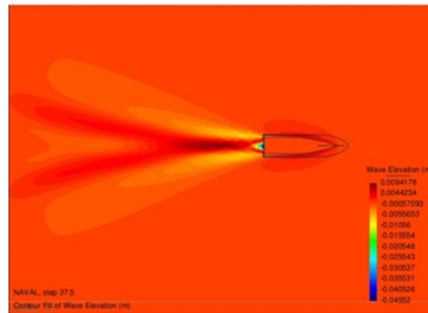
Figure 5. Wave Pattern of the Original Model Fn 1,356
