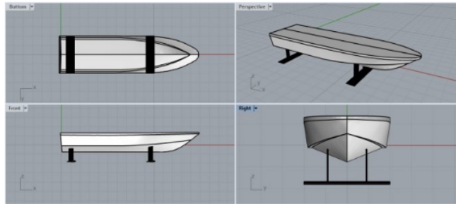
Figure 1. Pilot Boat 3D Modeling with foils
