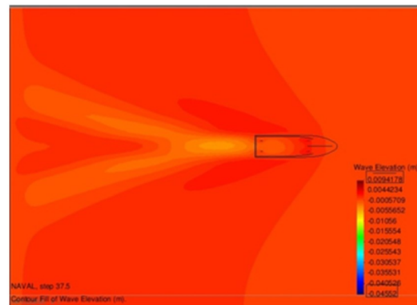
Figure 6. Wave Pattern of the 4L Foil angle of attack 5^\circ Fn 1,356
