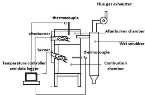
Fig. 1: Experimental rig.
