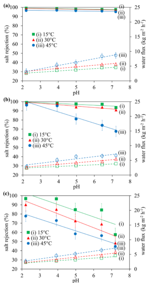
Fig. 10. Salt rejection (filled bullet) and water flux (open bullet) of DMDMS-TEOS silica membranes at NaCl concentrations of (a) 0.3 wt.% (b) 1 wt.% (c) 3.5 wt.%.
