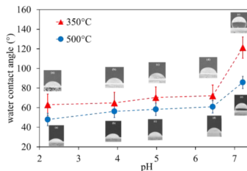
Fig. 2. The water contact angle of DMDMS-TEOS silica thin films coated on ceramic plates calcined at 350 °C and 500 °C as a function of pH.
