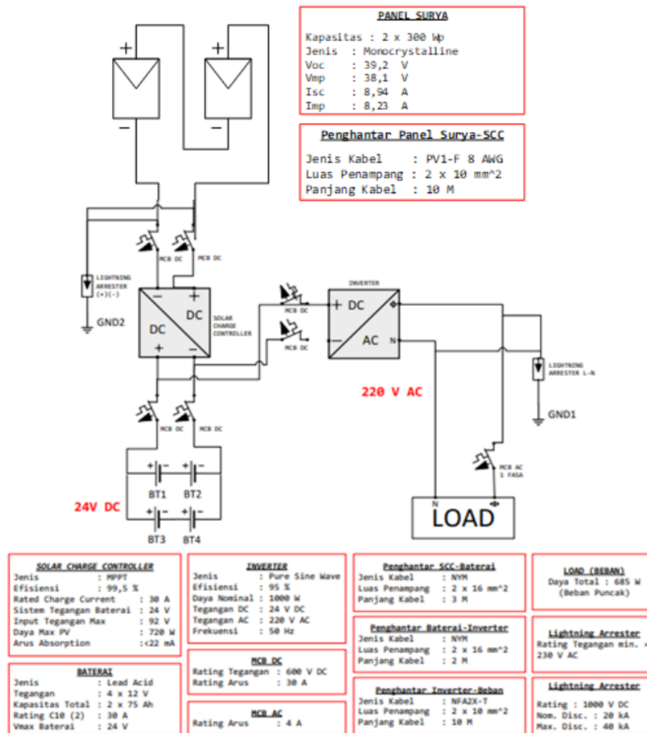
Figure 6. Detailed Engineering Solar on Power Plant System
