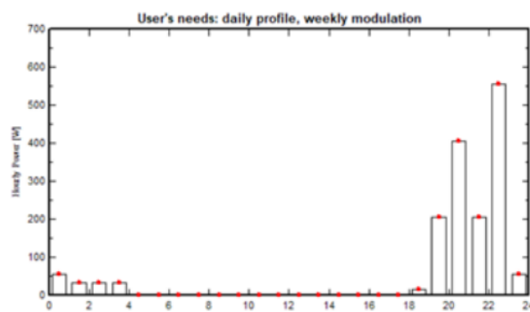
Figure 2. Daily Load Graph at Research Area
