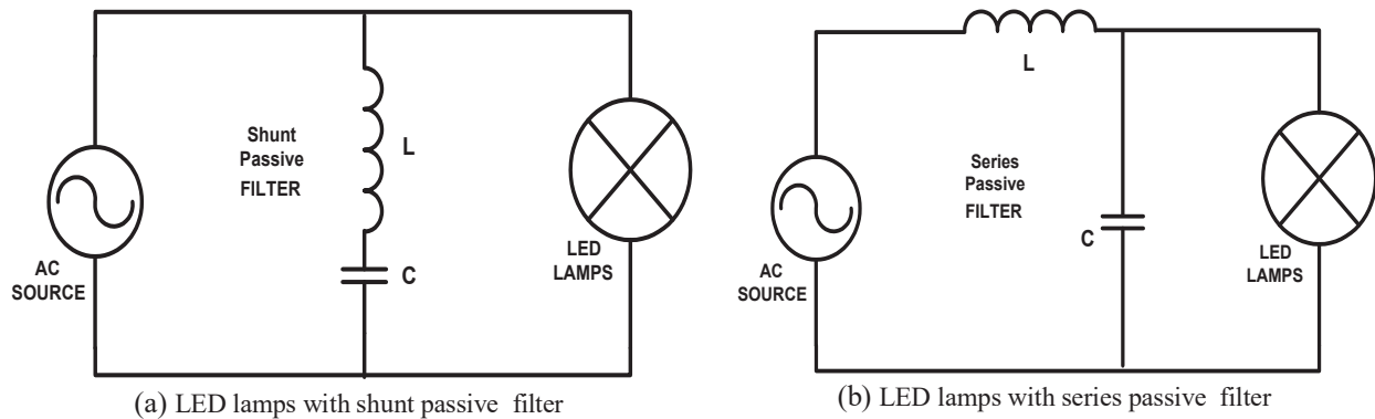
FIGURE 3. LED lamps with LC filter
