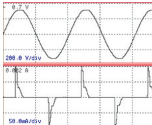
(b) Waveform LED lamp brand-Y
