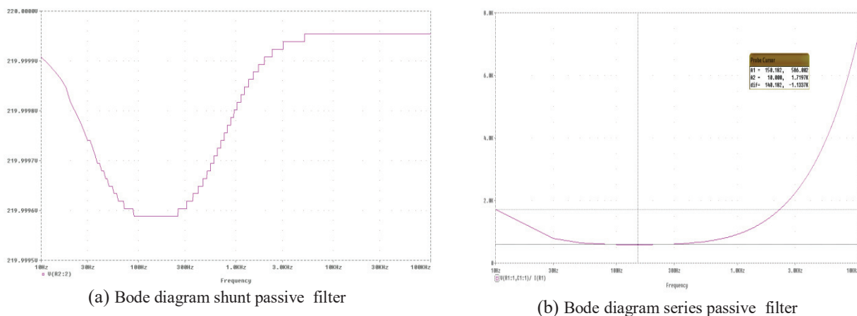
FIGURE 4. Bode diagram
