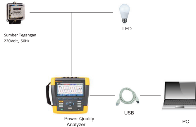
FIGURE 1. Harmonics measurement LED lamps
