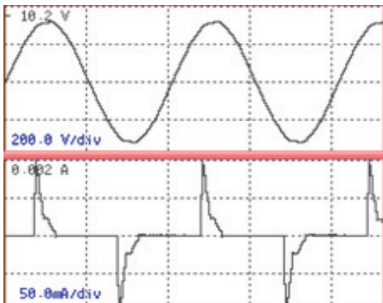
(a) Waveform LED lamp brand-X
