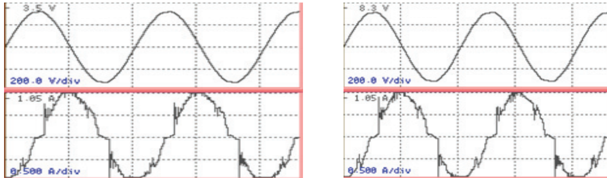
(a) Waveform LED lamp brand-X
