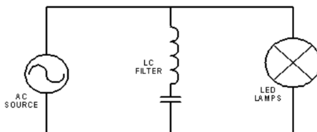
Figure 3. LED lamps with LC filter and AC source
