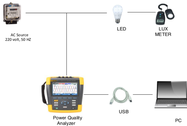
Figure 1. Harmonics & Lumen measurement LED lamps
