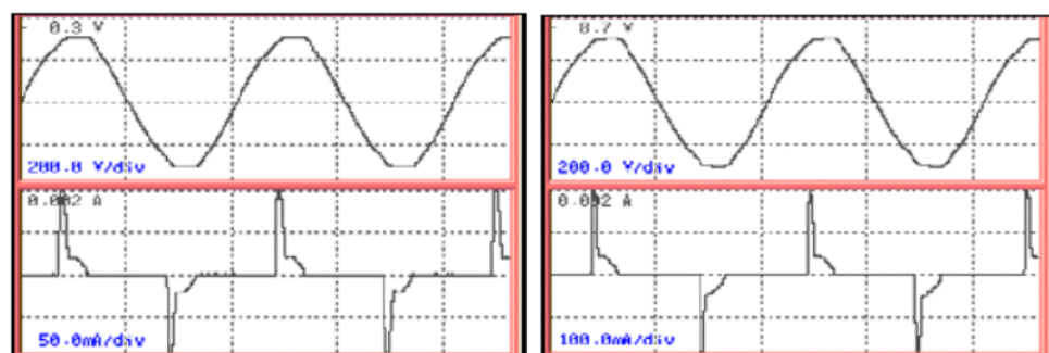
(a) Waveform LED lamp brand-A
