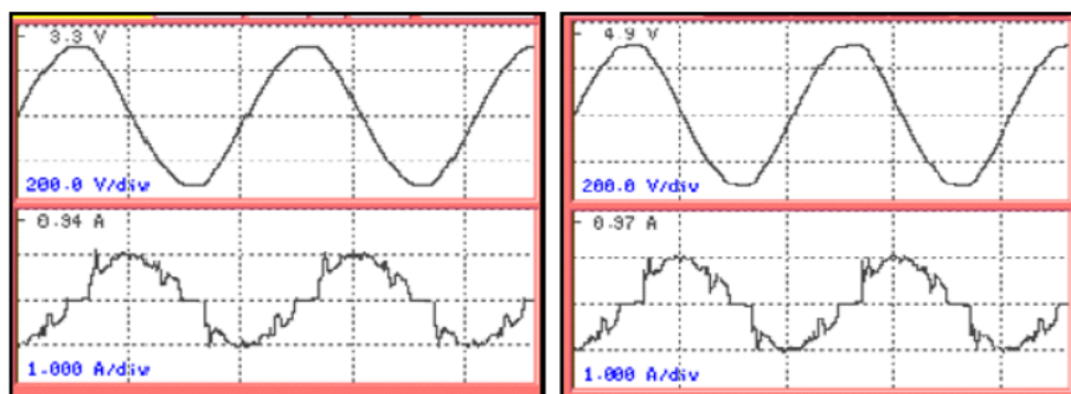
(a) Waveform LED lamp brand-A
