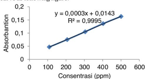
Fig 1: Calibration curve COD levels 108 ppm to 500 ppm.
