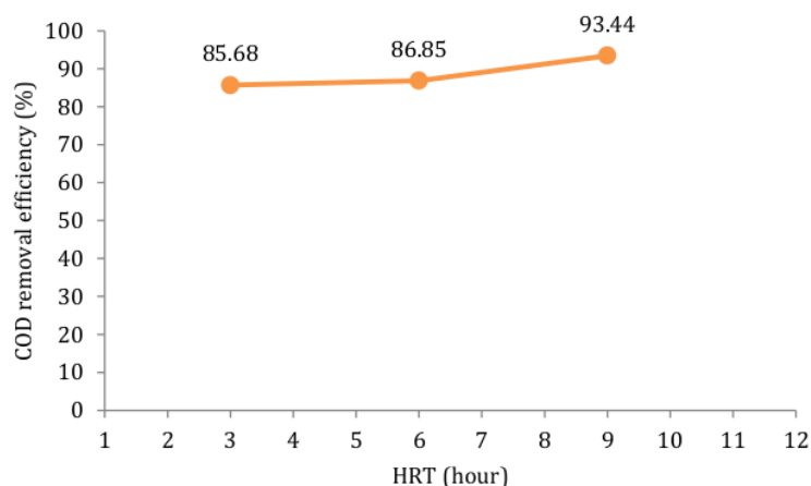
Figure 6. Results of the study on the percentage of fat COD removal in 3, 6, 9 hours HRT
