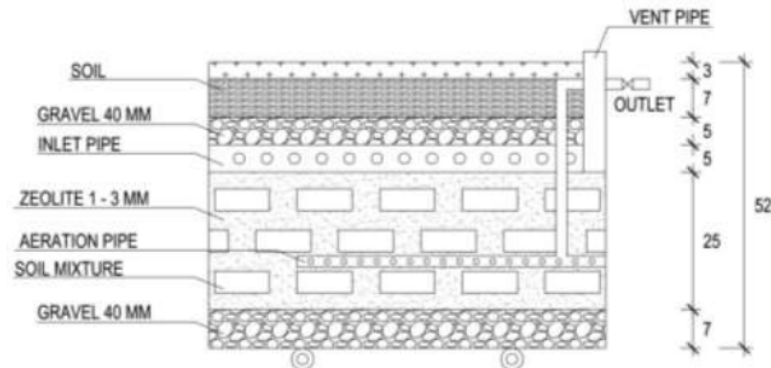
Figure 1. Multi Layer Soil system
