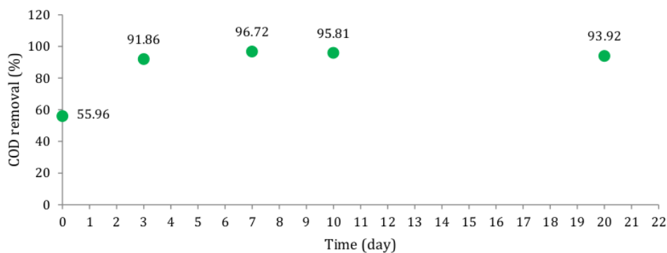
Figure 2. Graph of COD Removal Efficiency During Acclimatization
