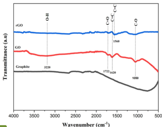
Fig. 3 FT-IR spectra of graphite, GO, and rGO.
