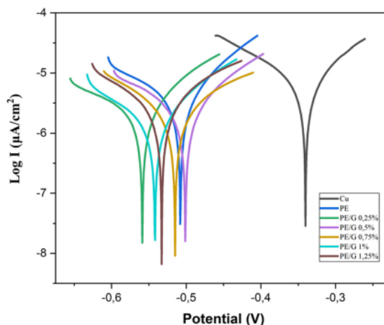
Fig. 9 Tafel plots of Cu, PE, PE/G 0.25%, PE/G 0.5%, PE/G 0.75%, and PE/G 1% measured in 3.5 wt% NaCl aqueous solutions.
