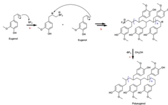
Fig. 1 Mechanism of eugenol polymerisation involving (a) initiation, (b) propagation and (c) termination stages. 12
