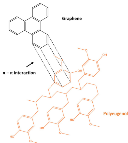
Fig. 5 Proposed interaction of polyphenol and graphene.
