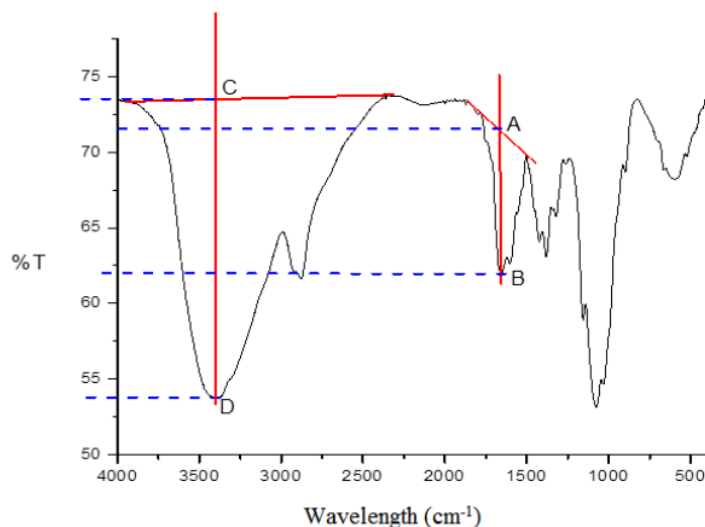
Figure 1. IR spectra for the determination of the degree of deacetylation using the base line method from the graph above, the degree of deacetylation is determined by the formula \%DD = 100 - \left[ \left( \frac{A_{1652}}{A_{3401}} \right) \times \frac{100}{1.33} \right] (Khan et al. , 2002)
