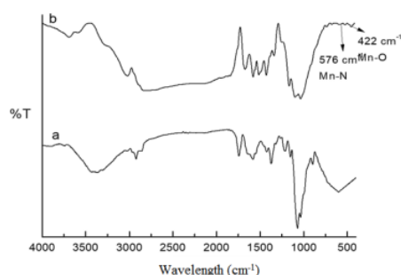
Figure 8. IR spectra of Mn(II)-Schiff base carboxymethyl chitosan-salicylaldehyde complex (a: Schiff base carboxymethyl chitosan-salicylaldehyde and b: Mn(II) Schiff base carboxymethyl chitosan-salicylaldehyde complex)
