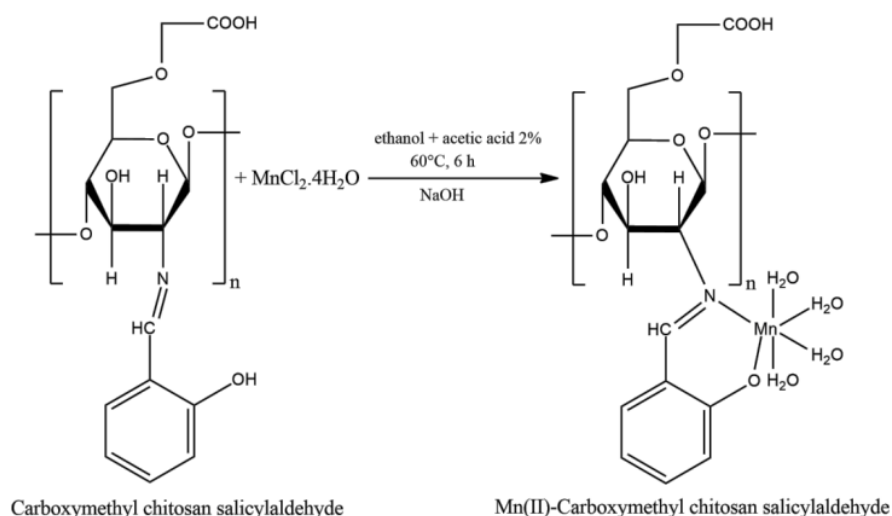
Figure 6. The reaction for the formation of the Mn(II)-Schiff base carboxymethyl chitosan-salicylaldehyde complex
