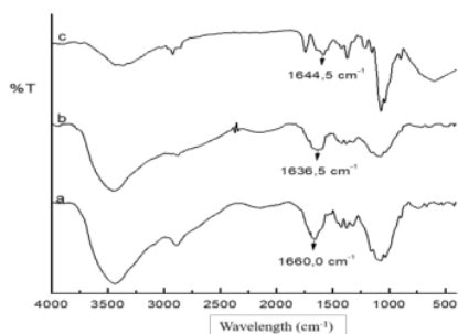
Figure 4. Infrared spectra of carboxymethyl chitosan, Schiff base carboxymethyl chitosan-benzaldehyde and carboxymethyl chitosan-salicylaldehyde (a:carboxymethyl chitosan, b:Schiff base carboxymethyl chitosan-benzaldehyde, c:Schiff base carboxymethyl chitosan-salicylaldehyde)
