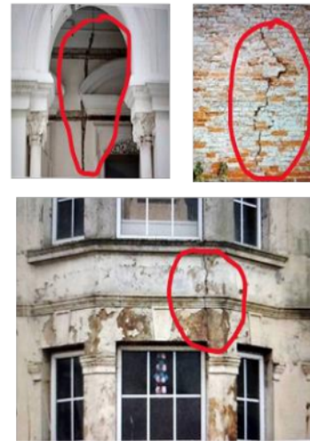
Fig. 1. Condition from the front side of the cracks of several ancient buildings in the old town of Semarang
