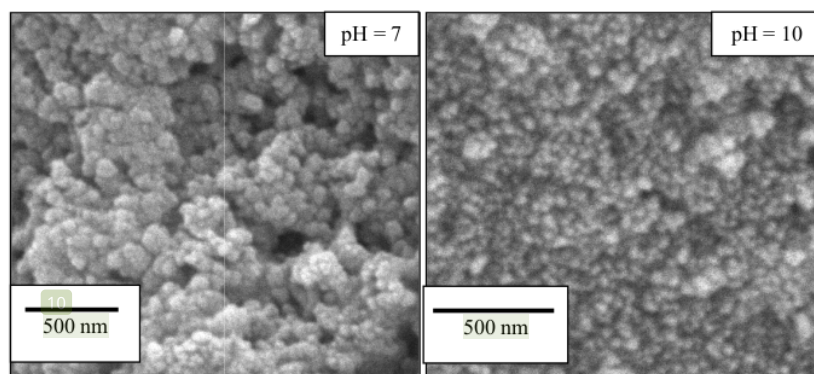
Figure 3. SEM images of nanoceria precipitated in (a) pH 7, (b) pH 10
