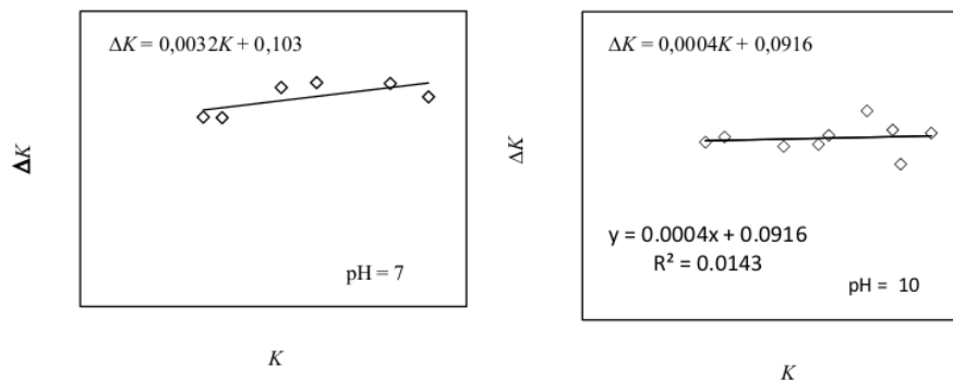
Figure 2. Williamson-Hall plots of nanoceria precipitated in (a) pH 7 and (b) pH 10
