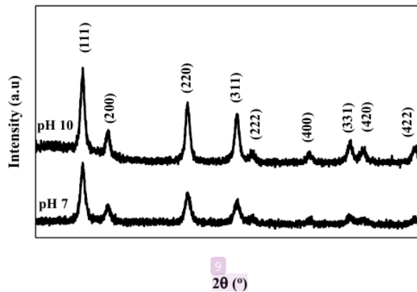
Figure 1. X-ray diffraction patterns of nanoceria precipitated in (a) pH 7, (b) pH 10
