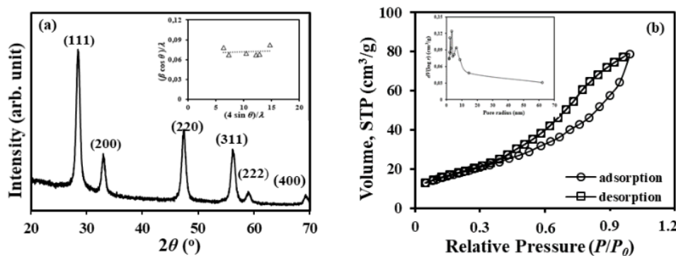
Fig. 1. (a). X-ray diffraction pattern and Williamson-Hall plot, (b). \text{N}_2 adsorption-desorption isotherm and the pore size distribution of ceria nanocrystal
