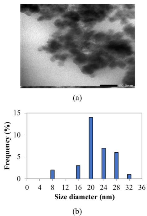
Fig. 4. (a) TEM image and (b) histogram SnNPs size in pure water medium.
