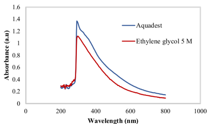
Fig. 3. The Colloidal absorption spectrum of SnNPs.
