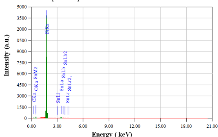
Fig. 6. EDX Spectrum of SnNPs.
