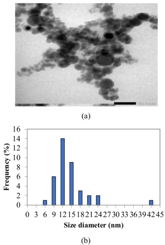
26 Fig. 5. (a) TEM image and (b) histogram SnNPs size in 5 M ethylene glycol medium.
