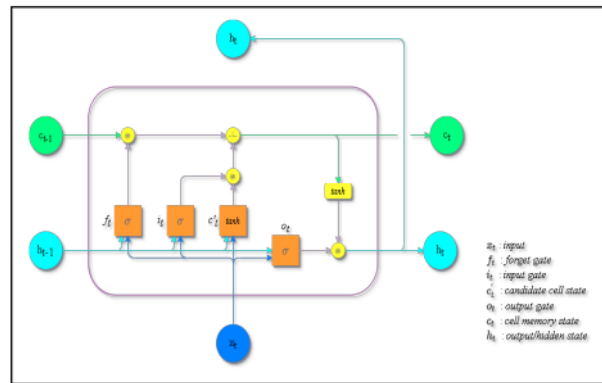
Fig. 1. LSTM Cell
