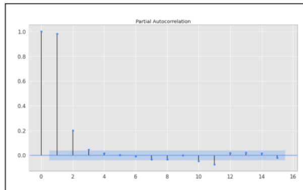
Fig. 2. PACF Plot of Crude Palm Oil Price
