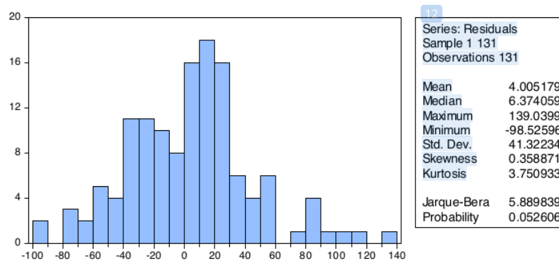
Gambar 3 Uji normalitas residual
