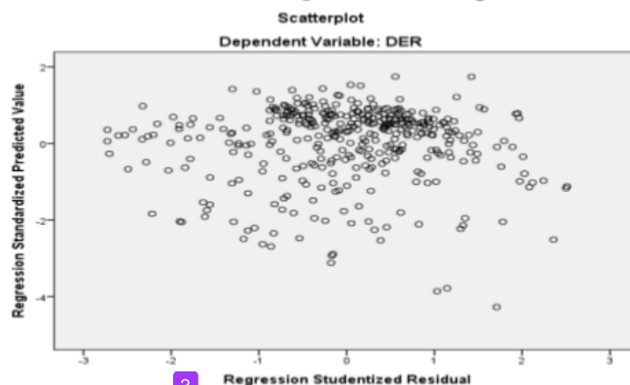
Gambar 4.5 Scatterplot (Model Regresi I)
