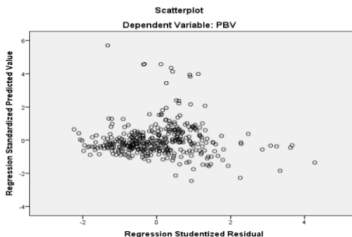
Gambar 4.6 Scatterplot (Model Regresi II)
