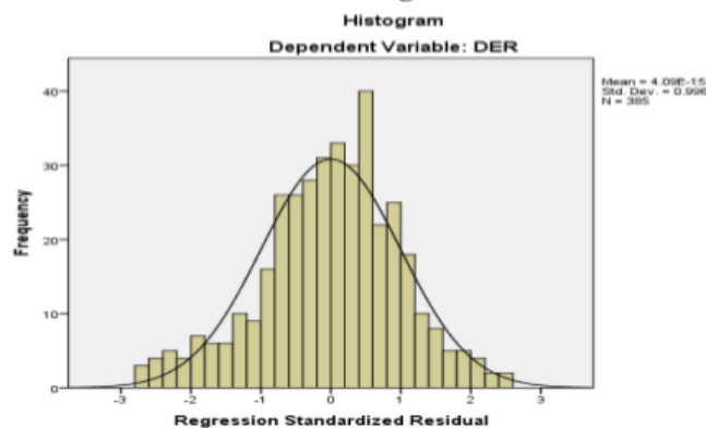
Gambar 4.2 Histogram
