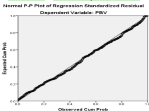
Gambar 4.3 P-P Plot Uji Normalitas
