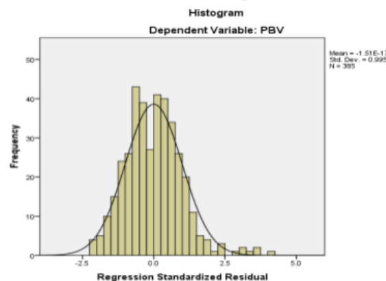
Gambar 4.4 Histogram
