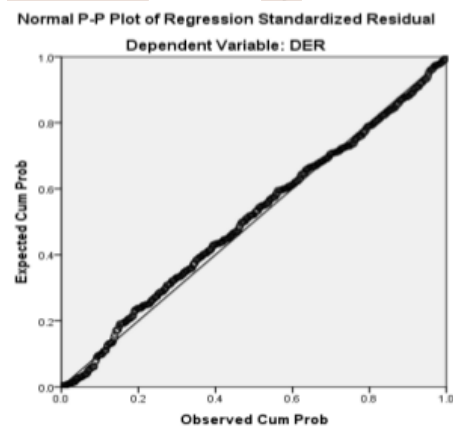
Gambar 4.1 P-P Plot Uji Normalitas
