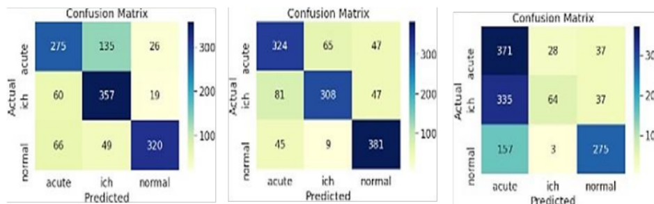
Figure. 8 Confusion matrix results for the three optimizer models in the ResNet-50 model: (a) RMSprop, (b) Adam and (c) SGD
