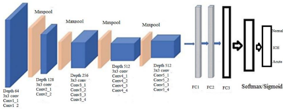
Figure. 9 VGG19 architecture
