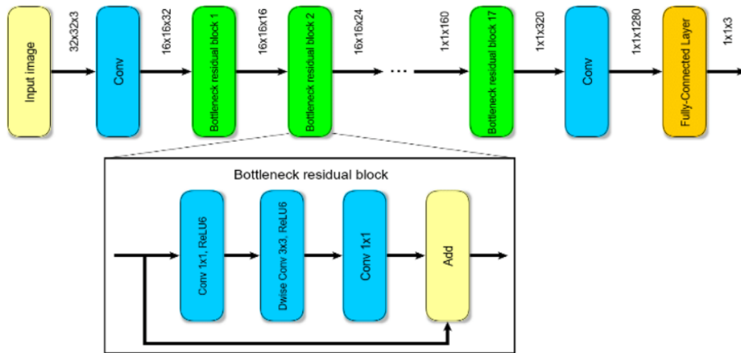
Figure. 11 Architecture of mobilenetV2
