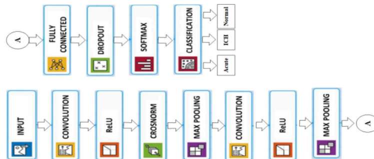
Figure. 3 CNN scenario 1 st model
