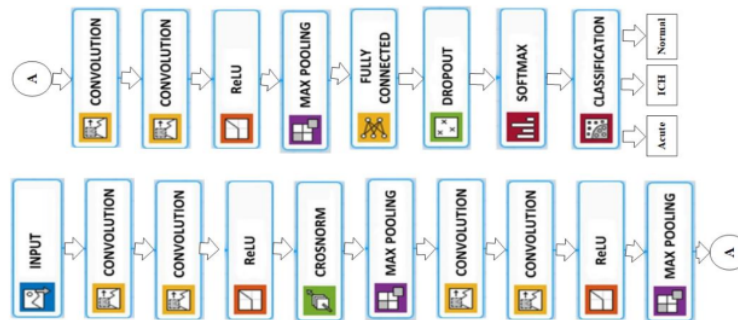
Figure. 4 CNN scenario 2 nd model / HCL-NN
