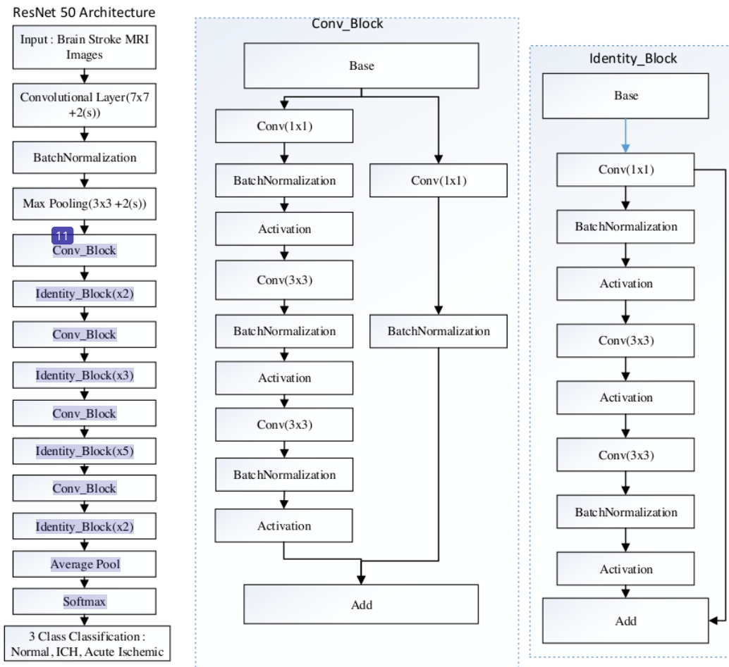
Figure. 7 ResNet-50 architecture block diagram
