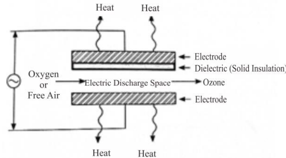
Figure 2. The principal of ozone generator by electrical discharge Source: JWWA, 1978
