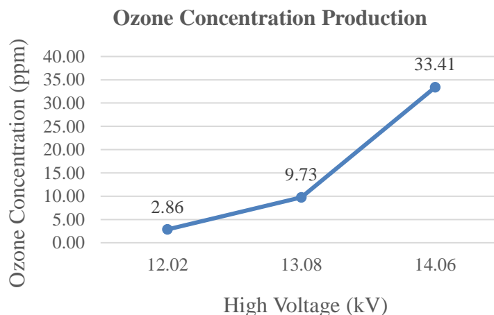
Figure 4. Ozone concentration production
