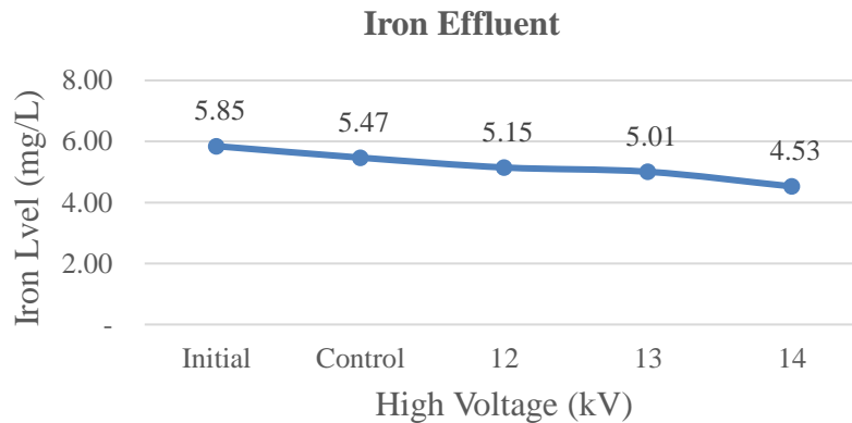
Figure 5. Iron effluent (before and after ozonation)
