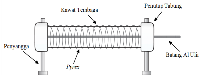
Figure 3. Dielectric Barrier Discharge Ozone Generator
