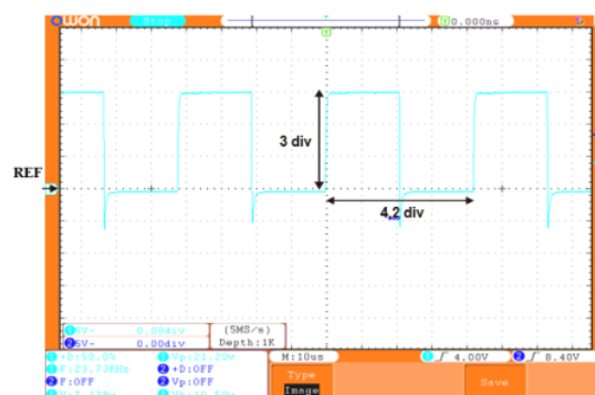
Figure 4. Output wave, V/div = 5 V, T/div = 10 \mu s/div.
