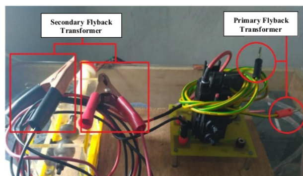
Figure 3. Modified flyback transformer.
