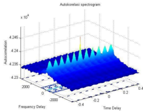
Figure 7. Vibration signal autocorrelation of faulty valve.
