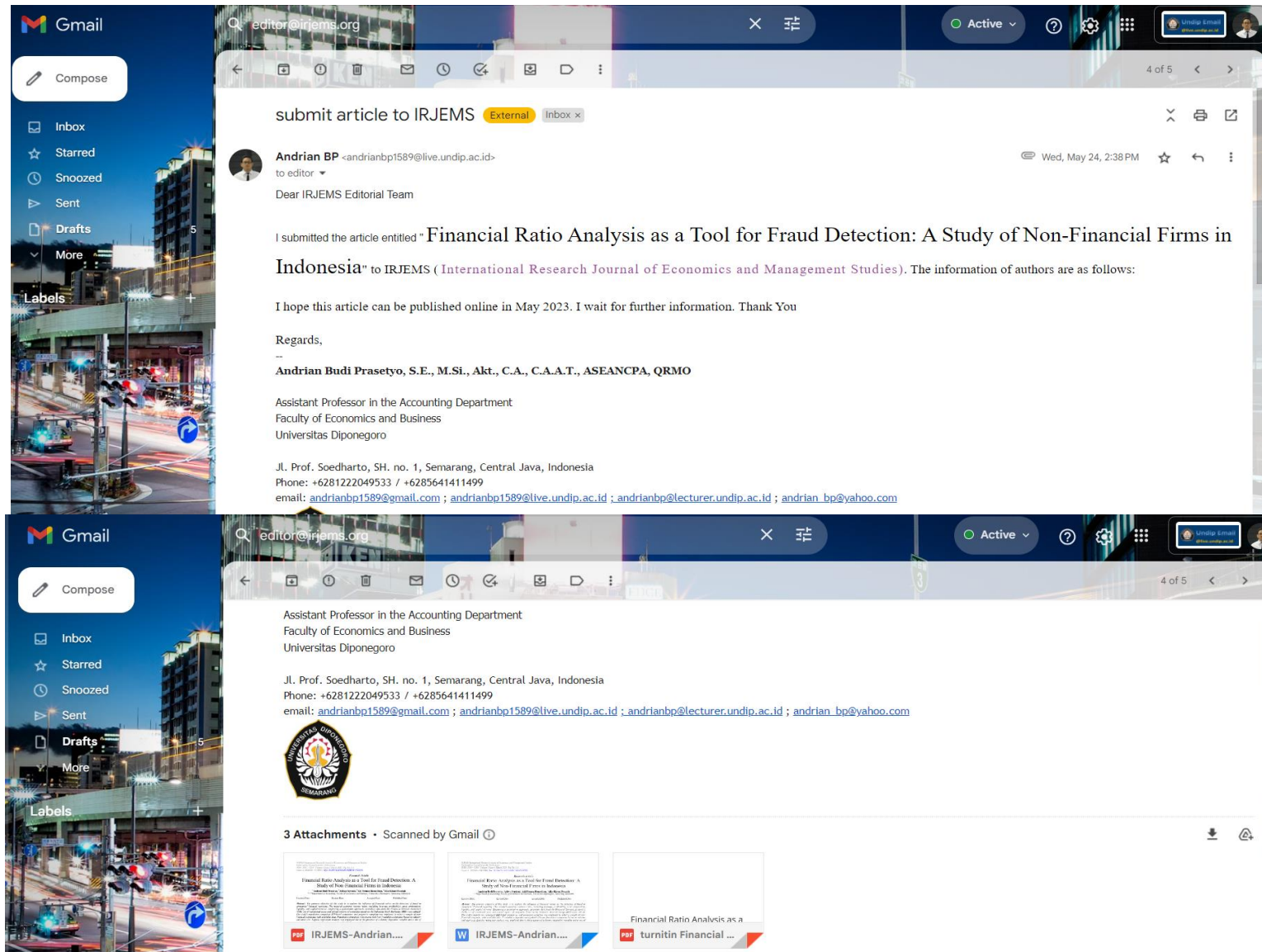
Figure 1. Submitting Article
