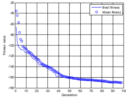
Gambar 8. Best dan mean fitness.
