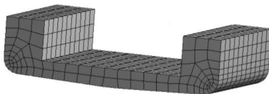
Gambar 3. Hasil meshing passive U-tube tank
