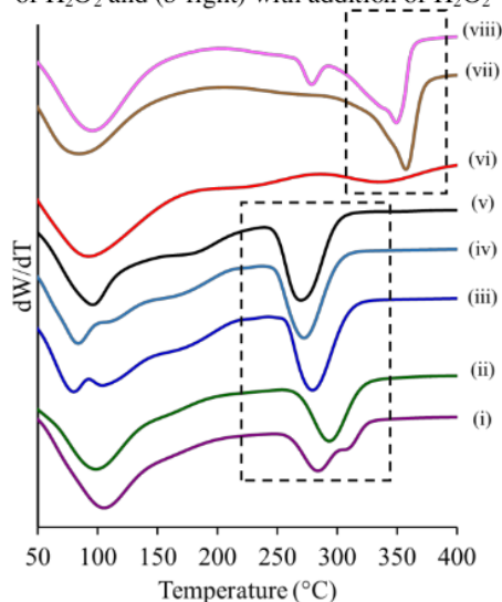
Figure 7. Differential of the TGA for samples prepared with varying Ni/Si molar ratios where (i) 5%, (ii) 10%, (iii) 25% (iv) 35% (v) 50% (vi) 10% with H 2 O 2 (vii) 25% with H 2 O 2 (viii) 50% with H 2 O 2
