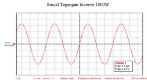
Gambar 4. sinyal tegangan output inverter 1000 watt
