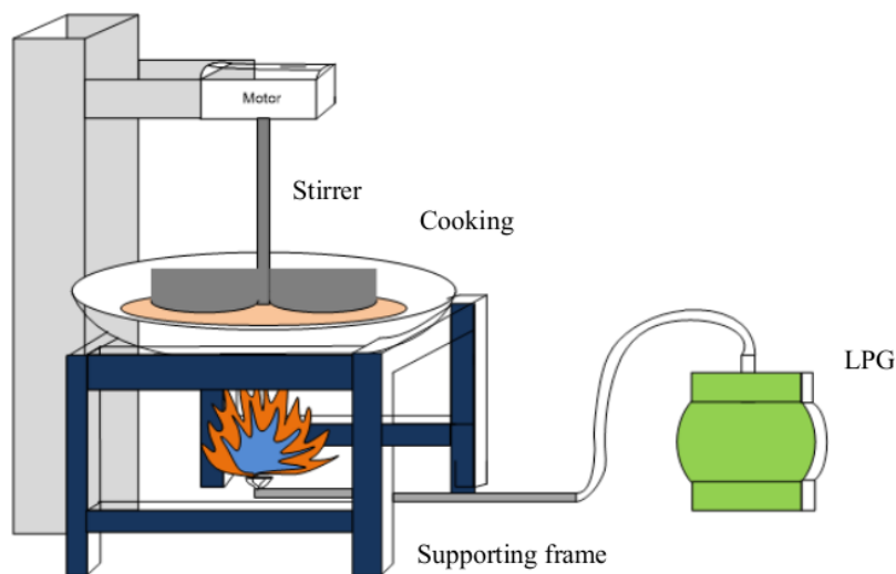
Figure 3. Design of the proposed equipment
