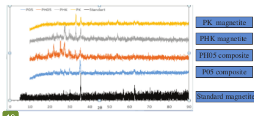
Fig. 1. X-ray diffraction patterns of magnetite and zeolite/magnetite composite.
