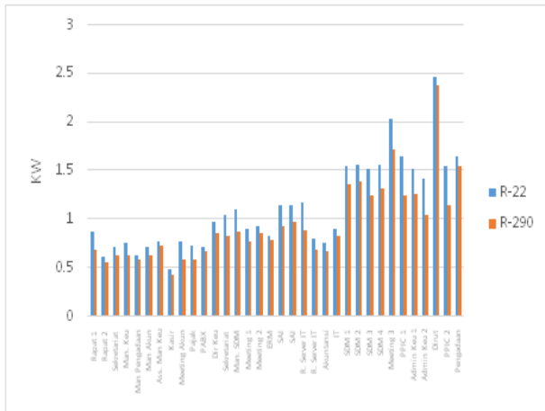
Figure 3: Power Consumption Comparison
