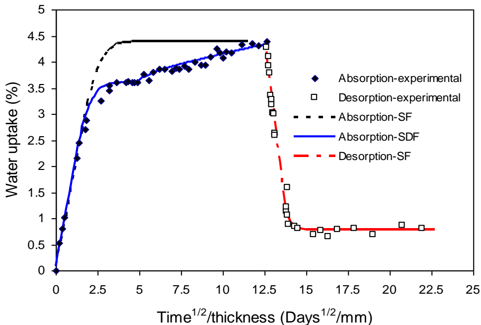
Figure 2 Water absorption and desorption of FM 73M
