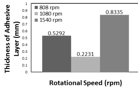
Fig. 16: The thickness of adhesive layer each tool
