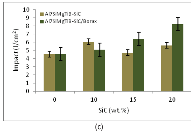
FIGURE 4. The price impact composite AlSi-Mg-TiB-SiC and AlSi-Mg-TiB-SiC/Borax
