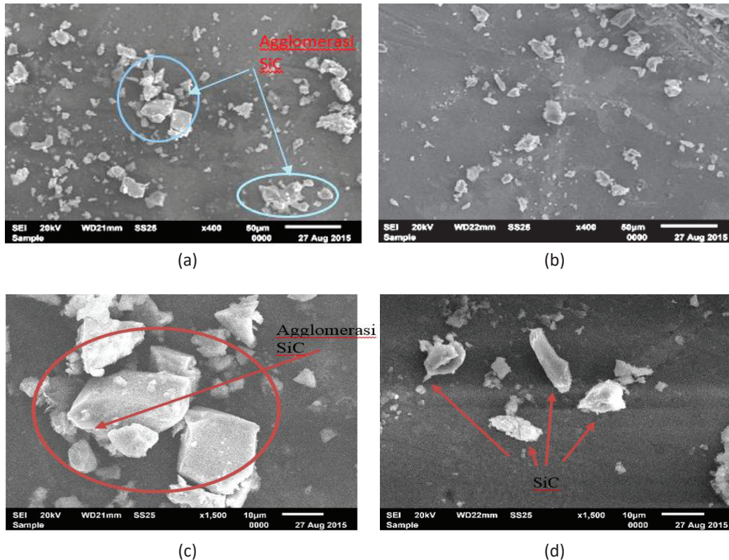
FIGURE 6. SEM Composite: Morphology (a) AISi-Mg-TiB-SiC 20 wt.% (b) AISi-Mg-TiB-SiC/Borax 20 wt%
