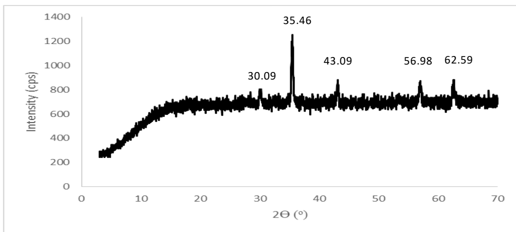
Fig. 3. Diffractogram XRD of magnetite after extraction treatment
