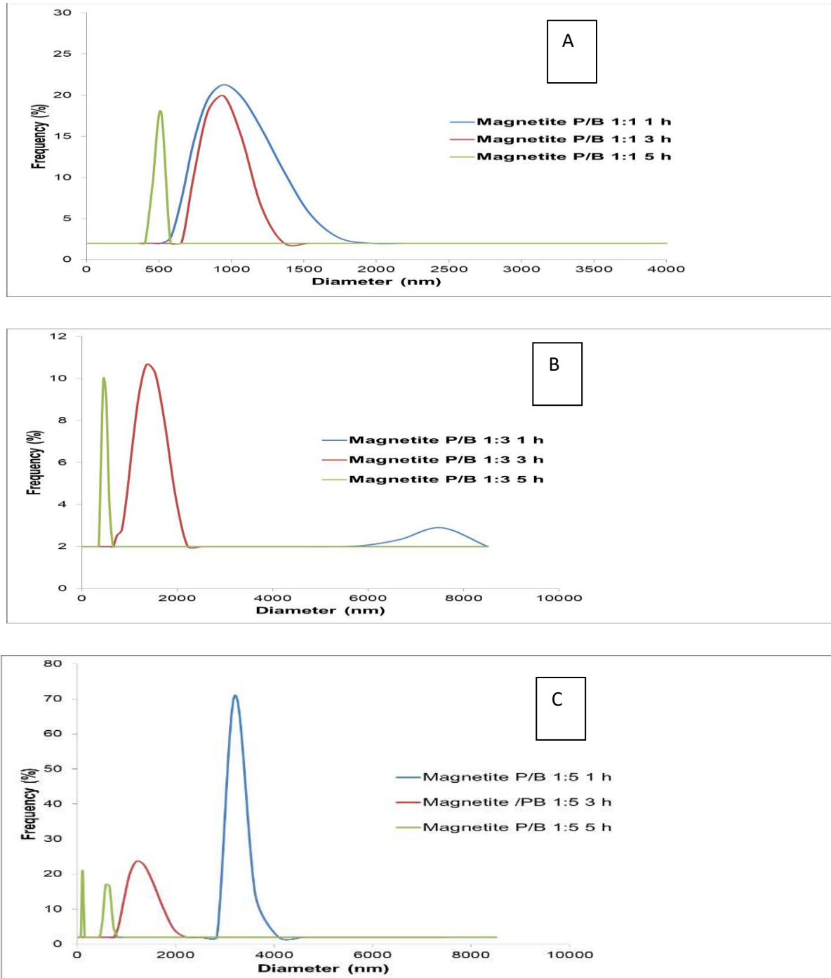
Fig. 7. Graph of magnetite size distribution on mass ratio magnetite:ball (P/B) 1: 1; 1: 3 and 1: 5
