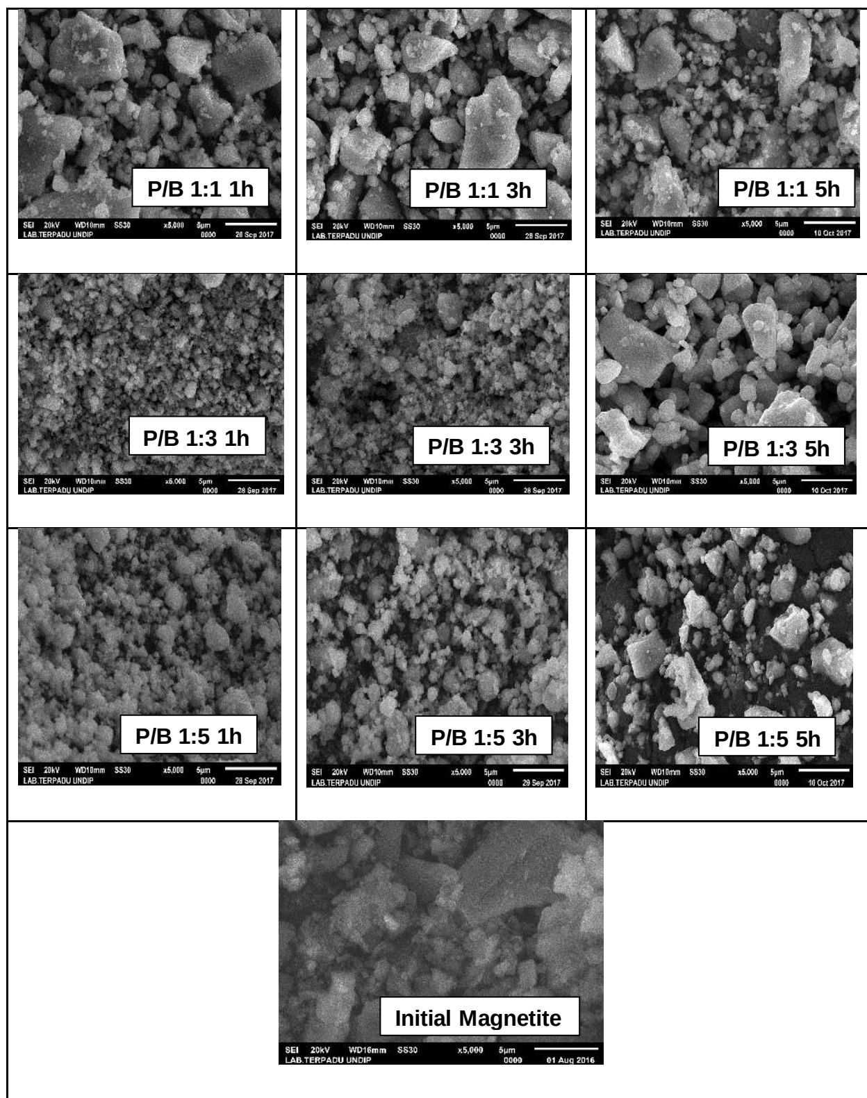
Fig. 8. Morphology of milled magnetite and initial magnetite by magnification 5000x
