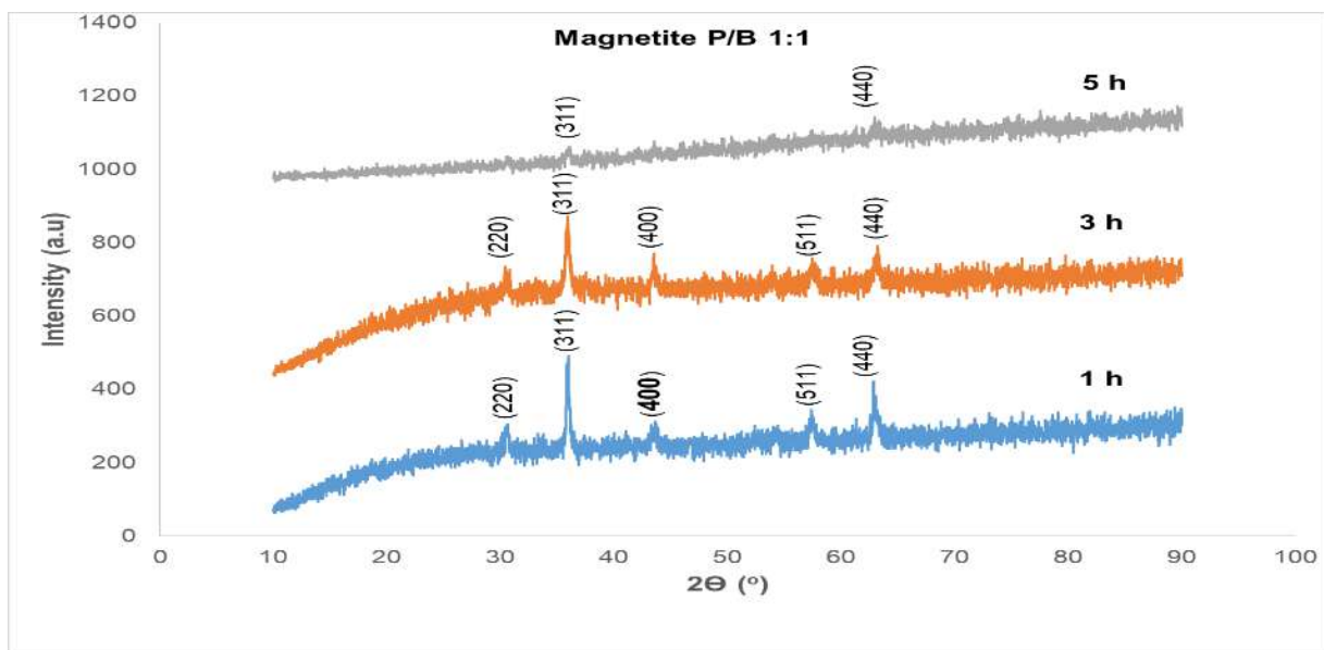
Fig. 4. Diffractogram milled magnetite by mass ratio of magnetite:ball (P/B) 1:1
