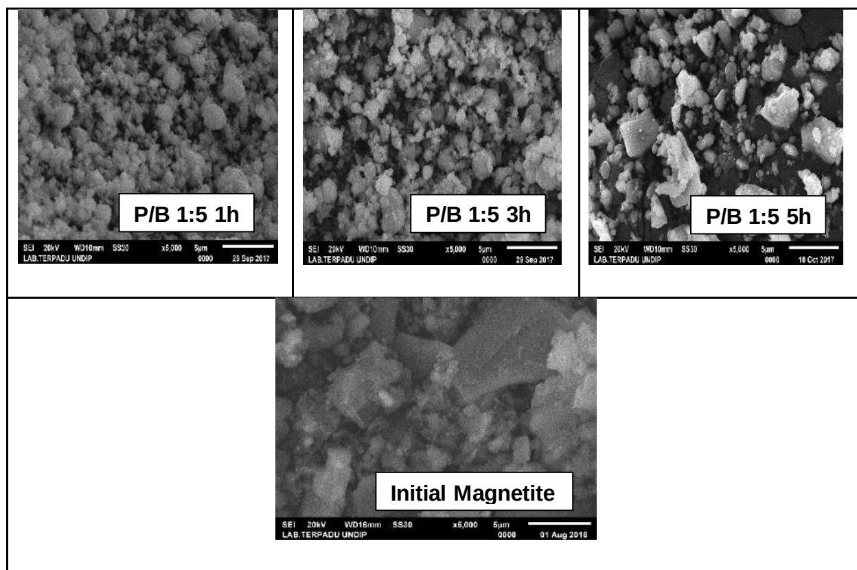
Fig. 8. Morphology of milled magnetite and initial magnetite by magnification 5000x
