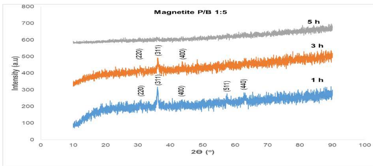
Fig. 6. Diffractogram milled magnetite by mass ratio of magnetite:ball (P/B) 1:5
