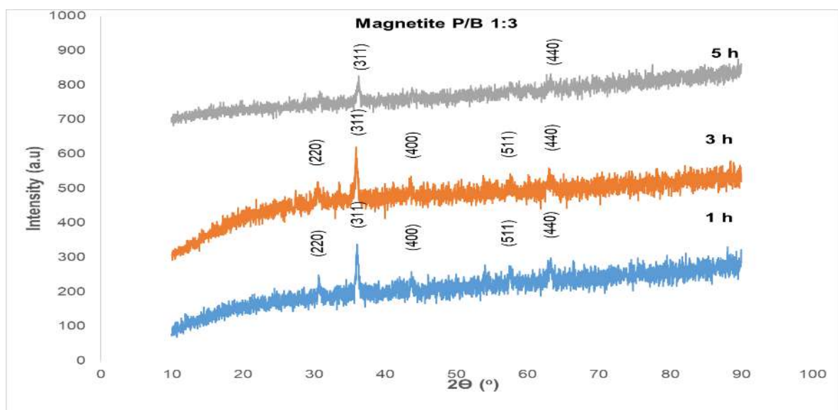
Fig. 5. Diffractogram milled magnetite by mass ratio of magnetite:ball (P/B) 1:3
