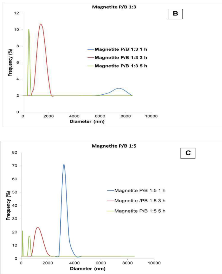
Fig. 7. Graph of magnetite size distribution on mass ratio magnetite:ball (P/B) 1: 1 (A); 1: 3 (B) and 1: 5 (C)
