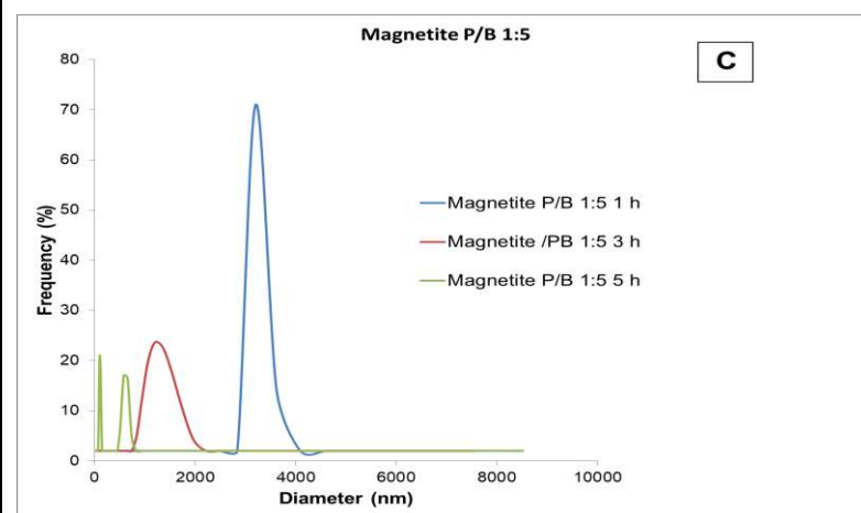
Fig. 7. Graph of magnetite size distribution on mass ratio magnetite:ball (P/B) 1: 1 (A); 1: 3 (B) and 1: 5 (C)
