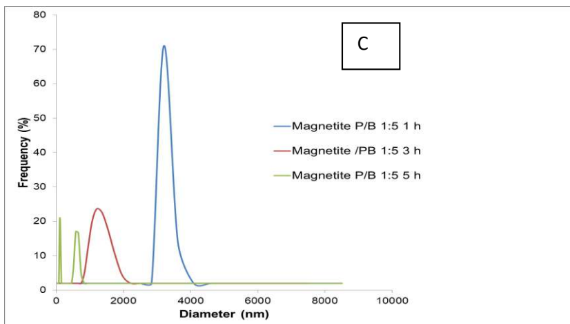
Fig. 7. Graph of magnetite size distribution on mass ratio magnetite:ball (P/B) 1: 1; 1: 3 and 1: 5
