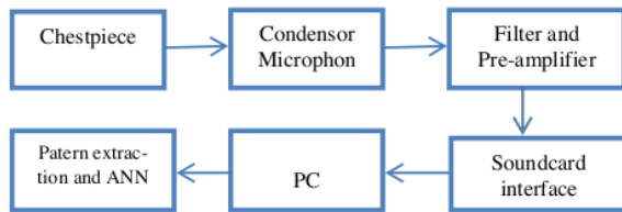
Fig. 3. Diagram block of the digital stethoscope design
