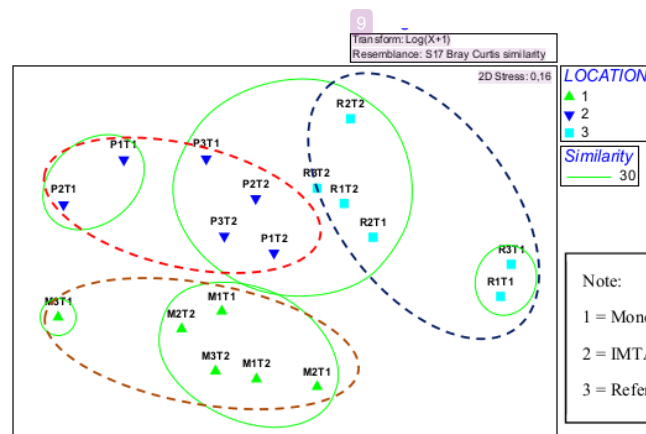
Figure 3. The 2D ordination of nonmetric multidimensional scaling (NMDS), indicating three groups based on sampling locations with 30% similarity values (green circle). Note: red, dashed circle: tendency of grouping/clustering at the stations of the IMTA site; brown, dashed circle: tendency of grouping/clustering at the stations of the monoculture site; blue, dashed circle: tendency of grouping/clustering at the stations of the reference site.
