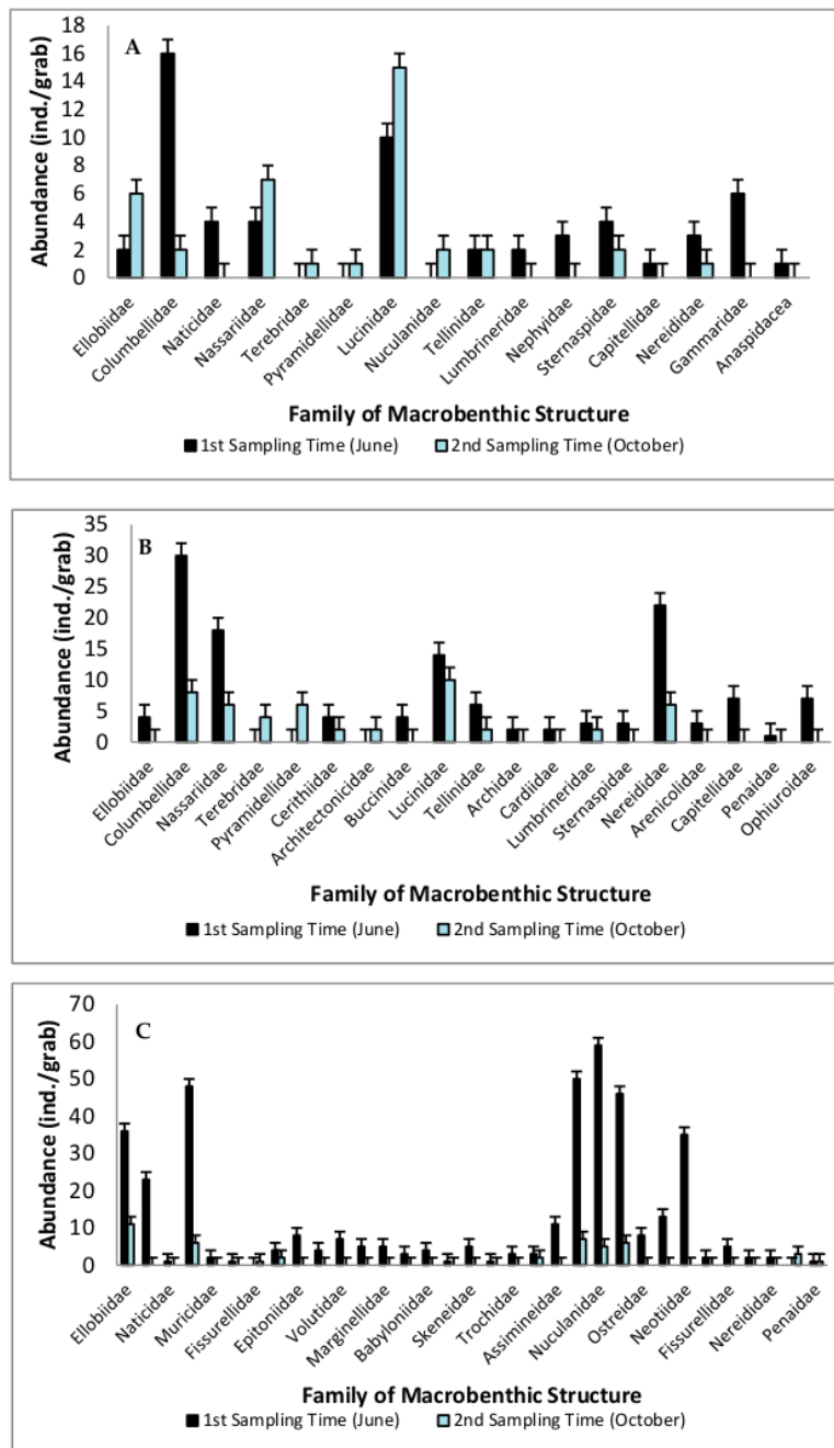
Figure 2. The structure of macrobenthos at (A) IMTA, (B) monoculture, and (C) reference site in different sampling time ( \pm SD).
