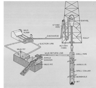
Gambar 5. Drilling string
