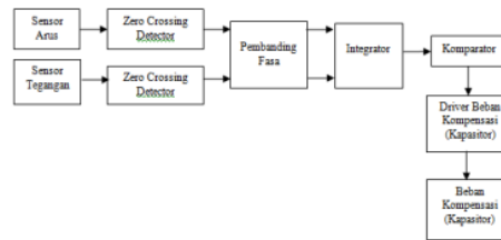
Gambar 12. Blok diagram
