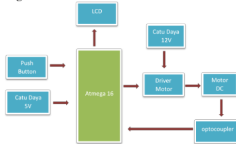
Gambar 6. Diagram blok
