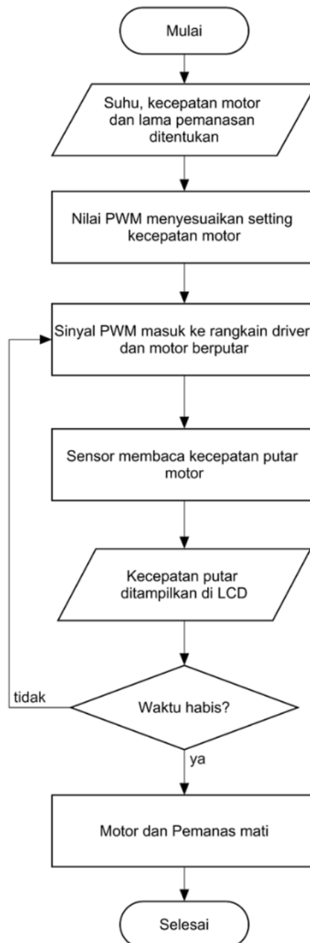
Gambar 8. Flowchart Sistem
