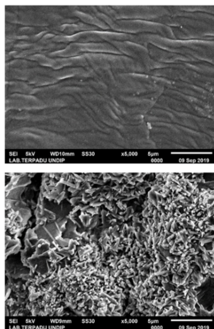
Fig. 10. SEM results referring to: (A) native \kappa -carrageenan; (B) \kappa -carrageenan treated by US/O_3 .
