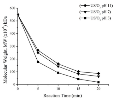
Fig. 5. An effect of pH on \kappa -carrageenan depolymerization (a temperature of 29 \pm 1^\circ C , O_3 concentration of 35 mg min^{-1}L^{-1} ).
