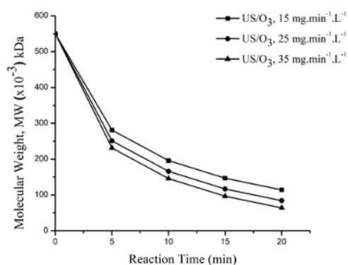
Fig. 4. An effect of the combined ultrasonication and ozonation on \kappa -carrageenan depolymerization (a temperature of 29 \pm 1^\circ\text{C} ; an initial pH value of 7).
