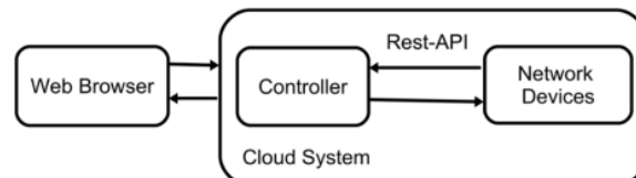
Figure 3. Network Automation System Design
