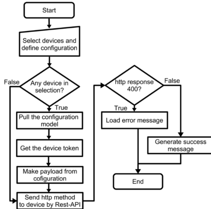
Figure 4. Network Automation Flow Chart
