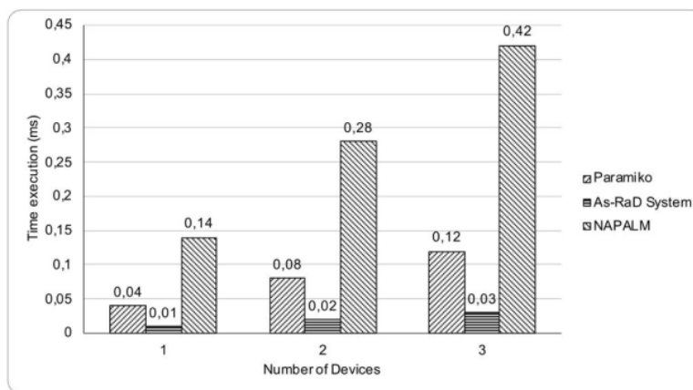
Figure 7. As-RaD System vs Paramiko and NAPALM
