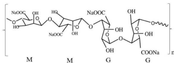
Figure 1. Structural characteristics of alginates: \beta -D-mannuronic acid (M) and \alpha -L-guluronic acid (G) residues.
