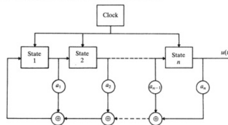
Gambar 2. Diagram state PRBS
