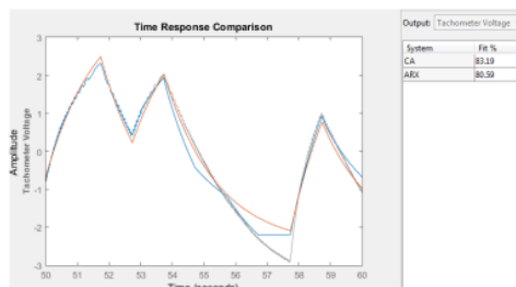
Gambar 6. Hasil Validasi Model
