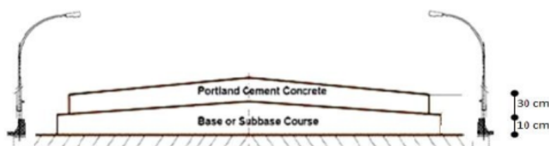
Fig. 2. Typical Cross Section of Rigid Pavement
