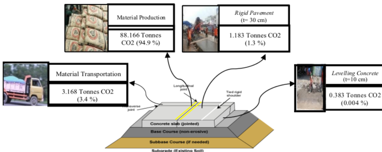
Fig. 7. Construction Process of Rigid Pavement
