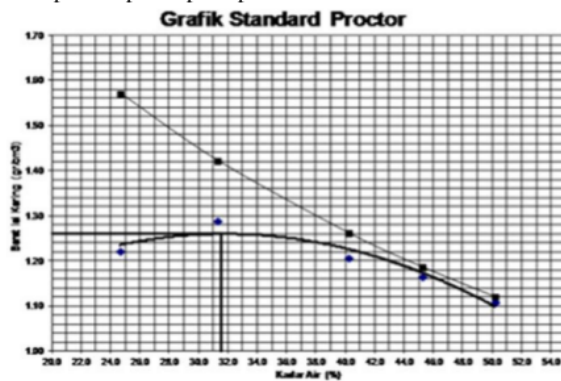
Gambar 1 Grafik standard proctor
