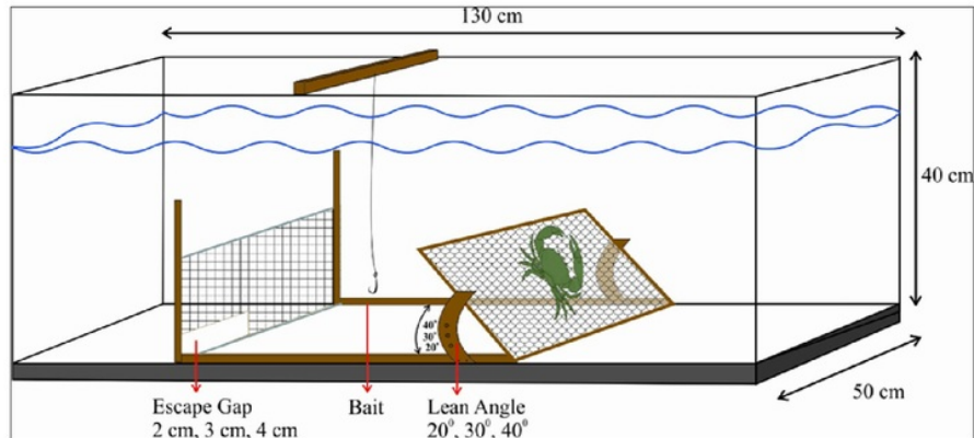
Figure 3. Experiment aquarium.
