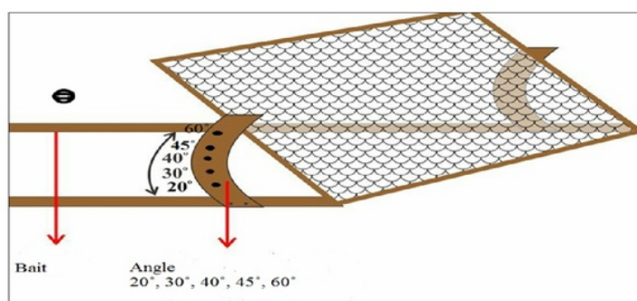
Figure 1. Funnel design.
