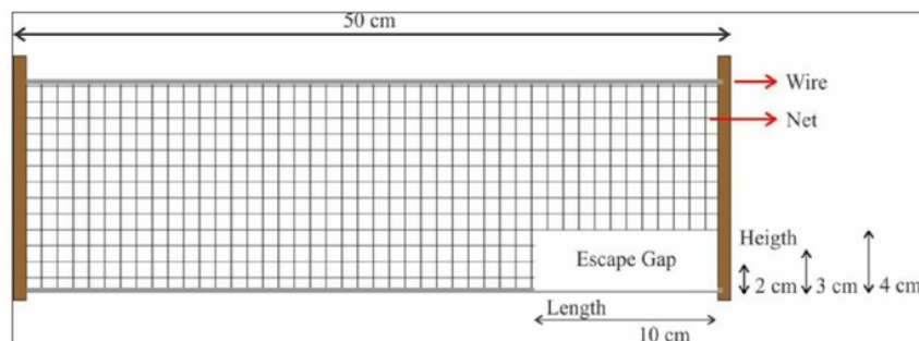
Figure 2. Escape vents size.
