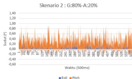
Gambar 7. Hasil pengujian Skenario 2 : gyroscope 80% - accelerometer 20%
