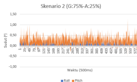
Gambar 6. Hasil pengujian Skenario 2 : gyroscope 75% - accelerometer 25%
